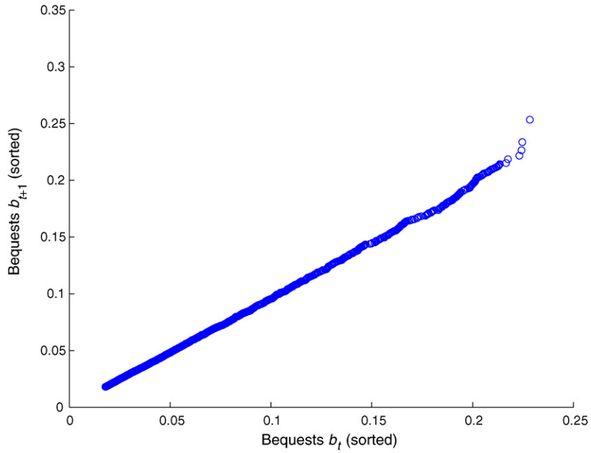
Fig. 1. Values of b_t (sorted) plotted against b_{t+1} (sorted). N = 100000 , only 10000 depicted.
