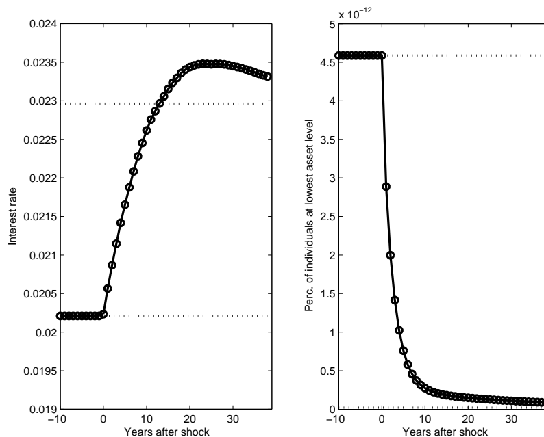
Figure 3: Transition from baseline economy ( \tau = 3.927\% ) to an economy with zero intermediation costs. Left graph: Interest rate. Right graph: Percent of individuals at lowest asset level.
