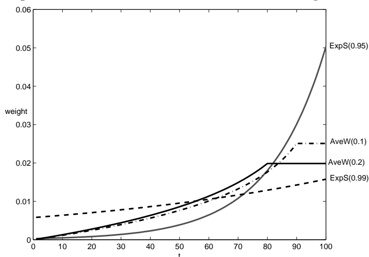
Figure 1: Weights attached to observations in AveW and ExpS forecasts for T = 100
