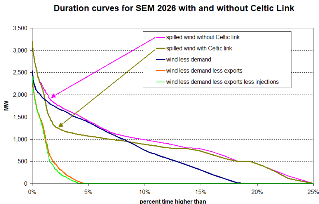
Figure 4 Duration curves with Celtic Link and comparisons of spilled wind without
