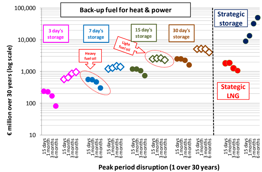
Figure 13. Lithuania: all measures, all scenarios (gas supply security levies)
