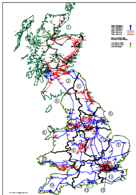
Figure 11: Demand Transmission Use of System charging zones in GB
