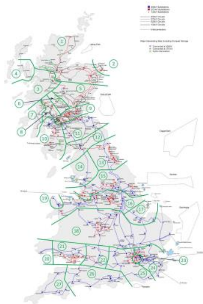
Figure 10: Generation Transmission Use of System charging zones in GB
