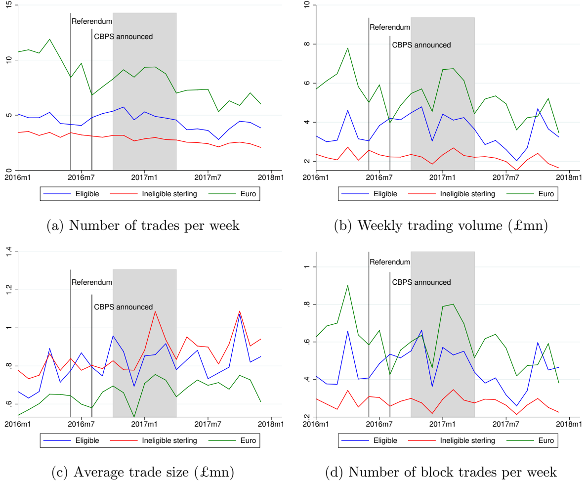
Figure 6: Measures of trading activity
