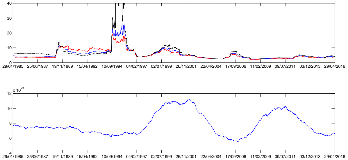
Figure 2: Plot of estimates for static scale (Bottom) and degrees of freedom (Top) with a 500 observations moving window. The top figure shows symmetric degrees of freedom \eta (Blue), asymmetric left tail degrees of freedom \eta_1 (Red) and asymmetric right tail degrees of freedom \eta_2 (Black). The estimated degrees of freedom are only reported if lower than 40.
