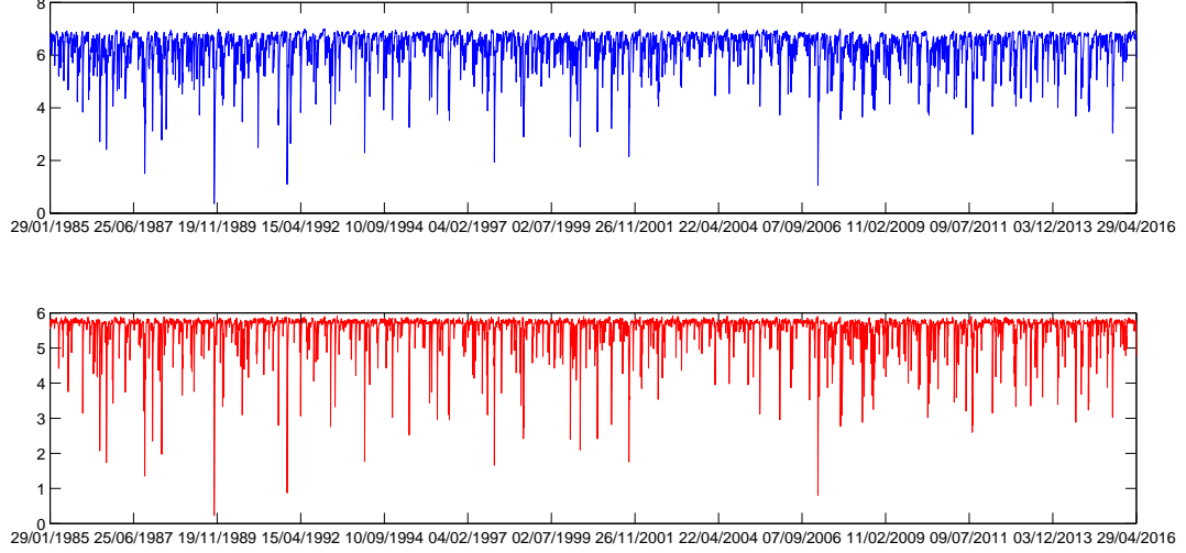
Figure 7: Fitted degrees of freedom of the Dow Jones Index Returns in the symmetric case (Top), \hat{\eta}_{t|t-1} , and for the Lower Tail in the asymmetric case (Bottom), \hat{\eta}_{1t|t-1} \bar{\eta}_{t|t-1} .
