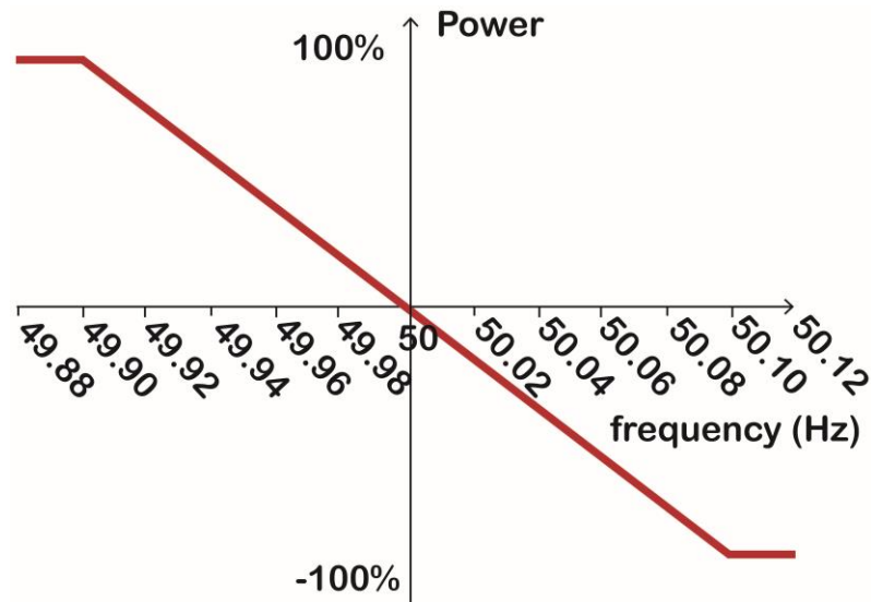
Fig. 3: Droop control signal for FCR-N in the Nordics
